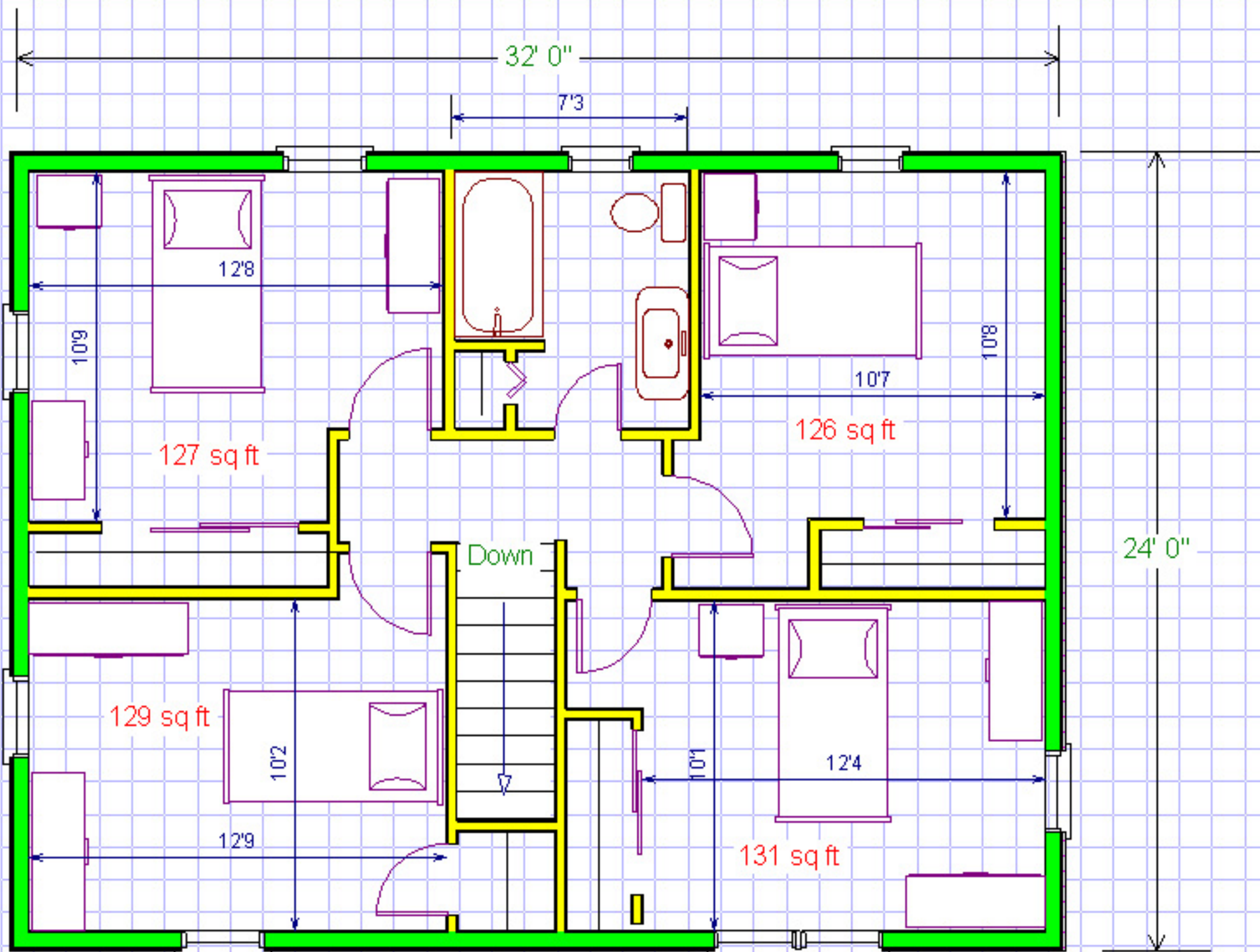
Cape-Colonial. 4 equally sized bedrooms, 1 bathroom.
